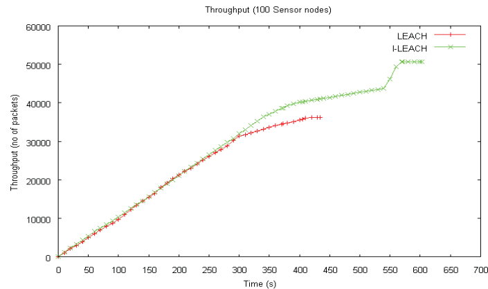
Fig. 6 Throughput comparisons
