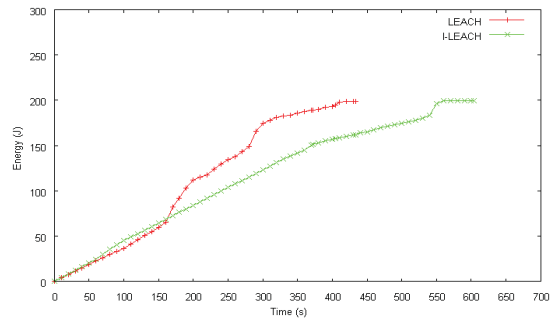
Fig. 5 Life time comparisons
