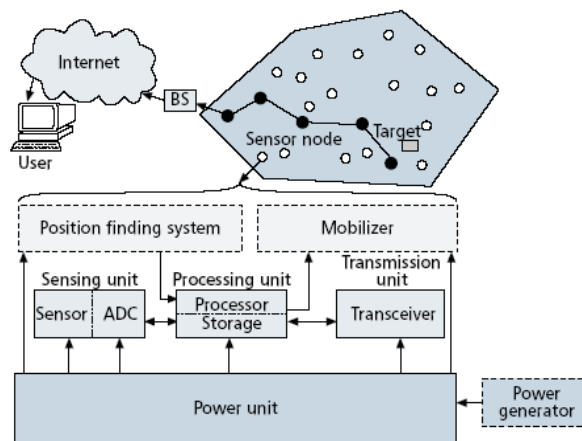
Fig. 2 Components of sensor node and WSN architecture
