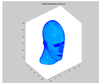
Fig1. Crust algorithm
