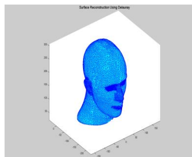
Fig2. Delaunay algorithm
