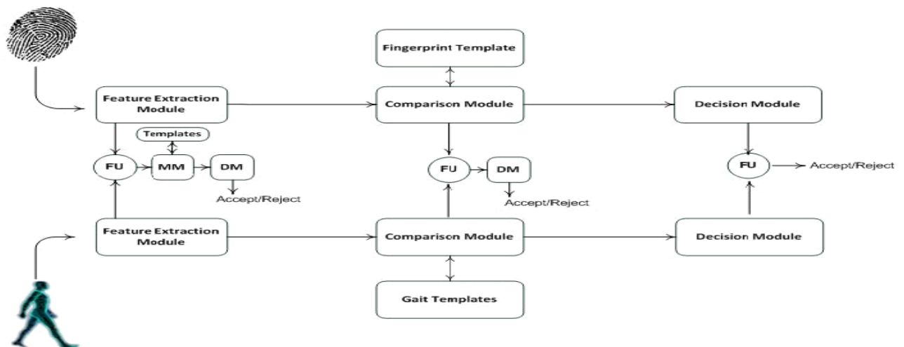
Figure 4: Different fusion levels
