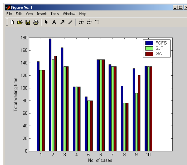
Figure 1 Results of various scheduling algorithms
