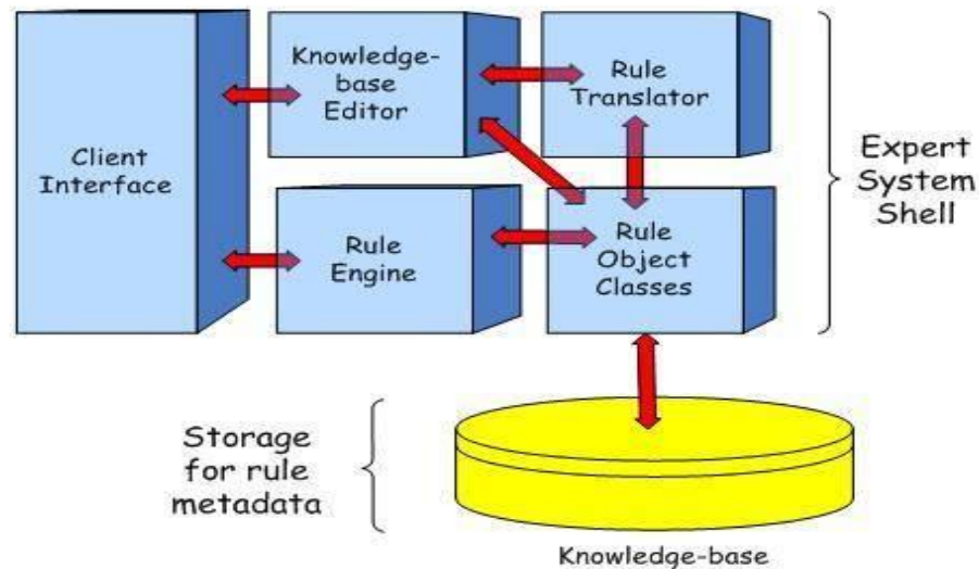
Figure 2 - Expert System Architecture
